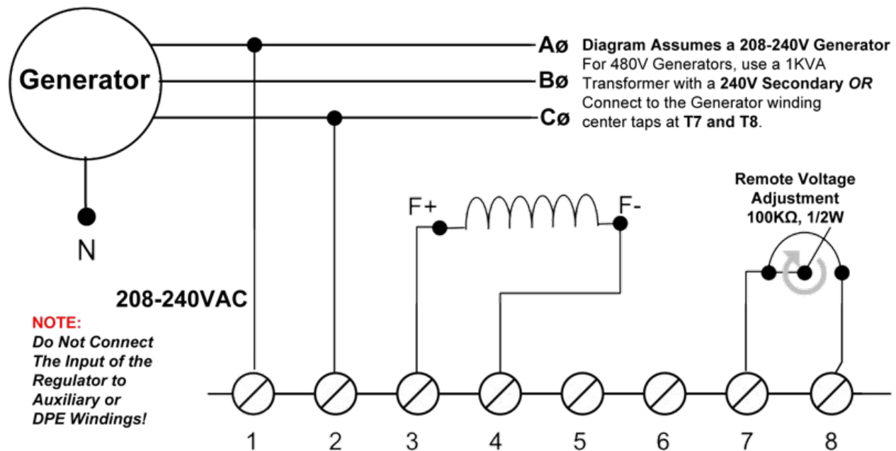
XR500D-300 Universal Voltage Regulator
